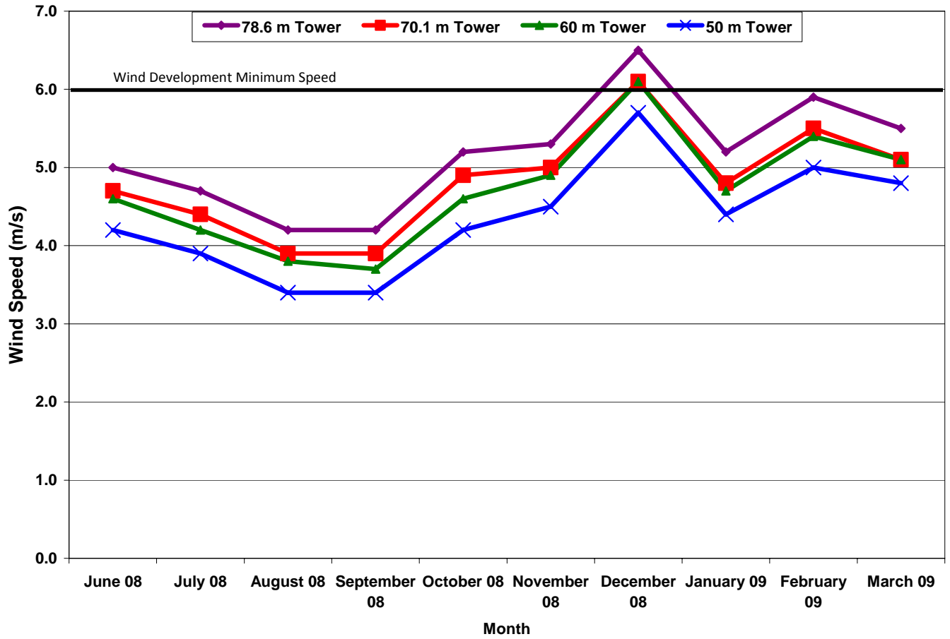
Figure 1: Average Monthly Wind Speed
