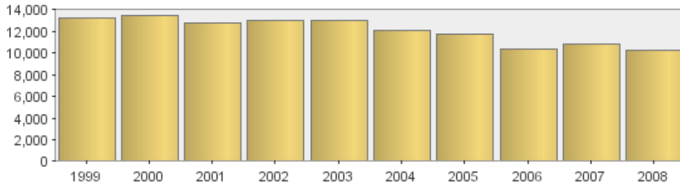
Crashes, 1999-2008
