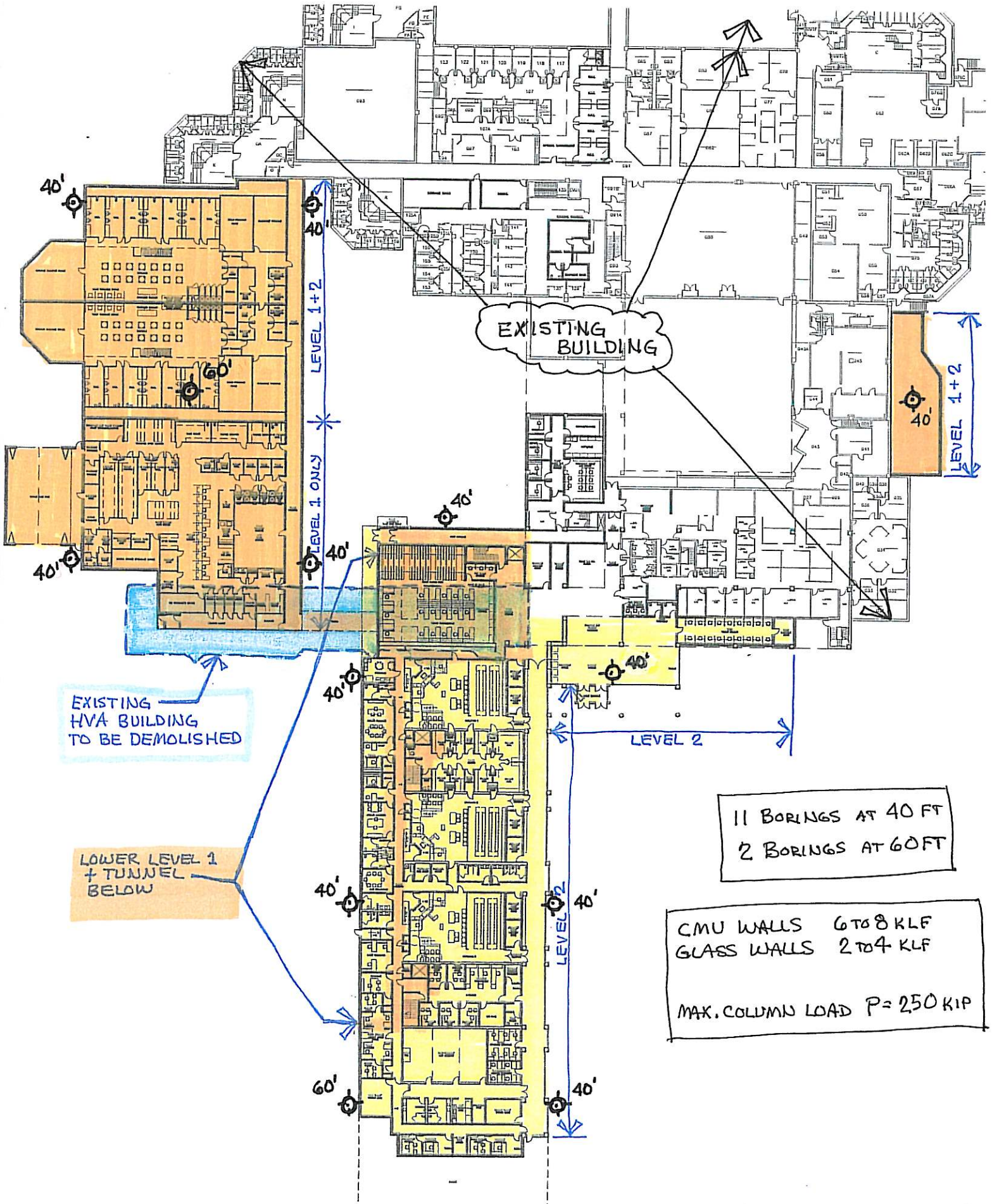
1 COMPOSITE FLOOR PLAN - LEVEL 1 + LEVEL 2 1/32" = 1'-0"
